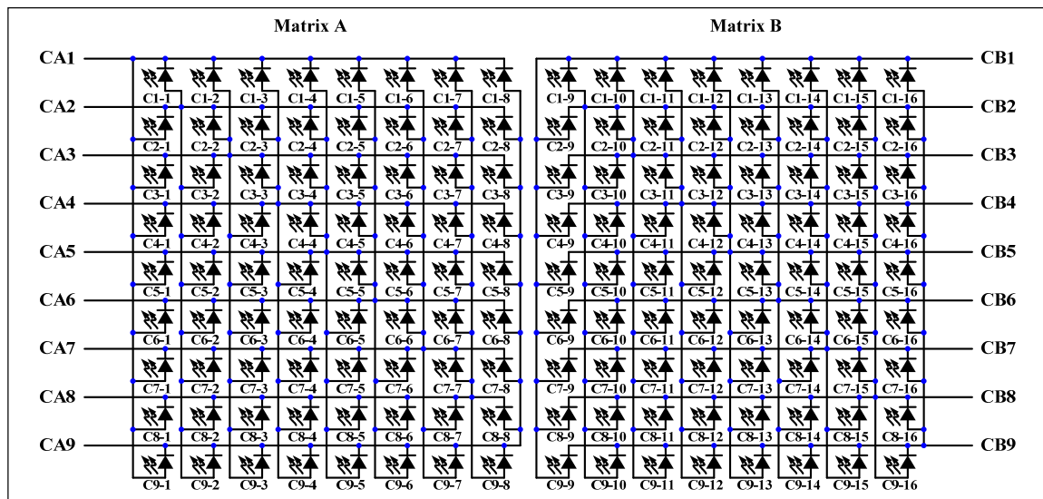
Figure 8 LED array
