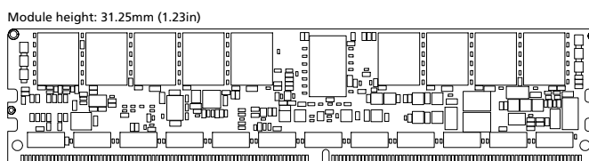
Figure 1: 288-Pin NVDIMM Decatur Two
