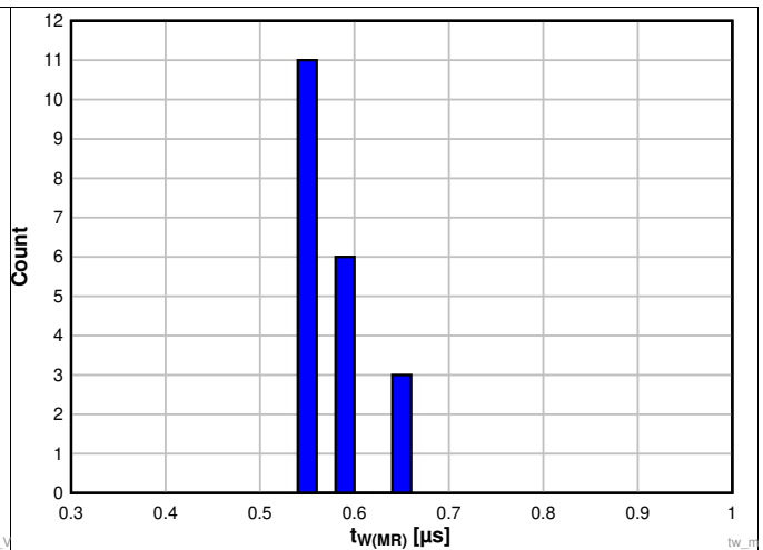
Figure 21. Manual Reset Pulse Width Histogram for TPS3823A-33 Devices at -40°C (Unit Count = 20)
