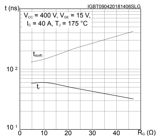
Figure 18. Switching times vs gate resistance
