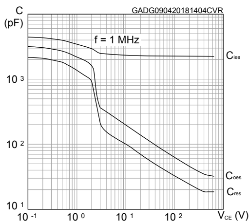
Figure 11. Capacitance variations
