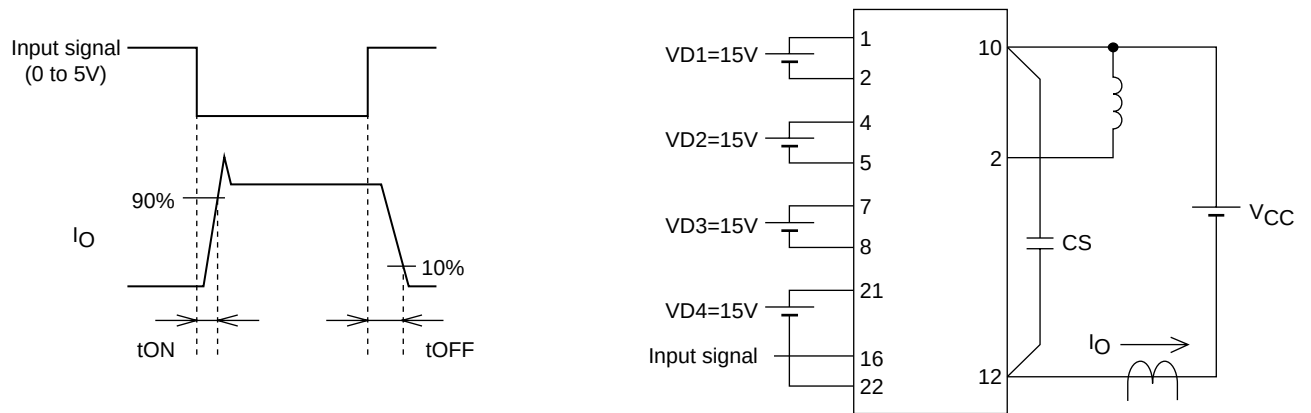
Fig 6: Switching Time
