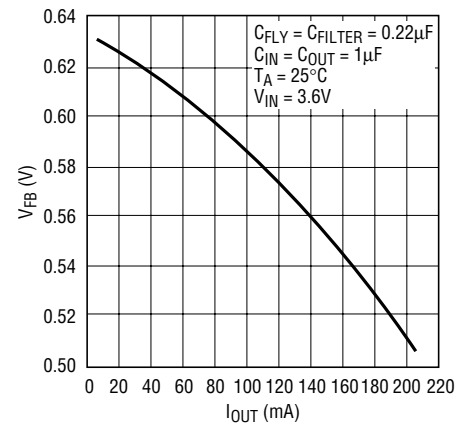
Feedback Voltage vs I_{\text{OUT}}
