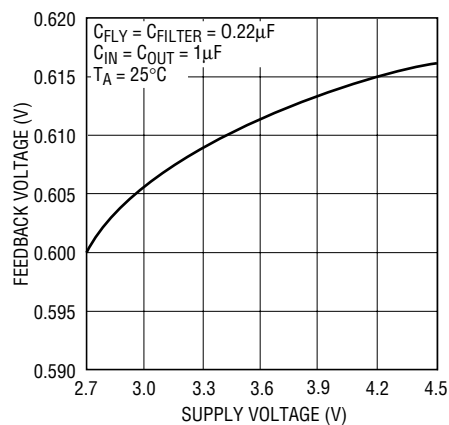
Feedback Voltage vs Supply Voltage I_{\text{OUT}} = 100\text{mA} , V_{\text{OUT}} = 4\text{V}
