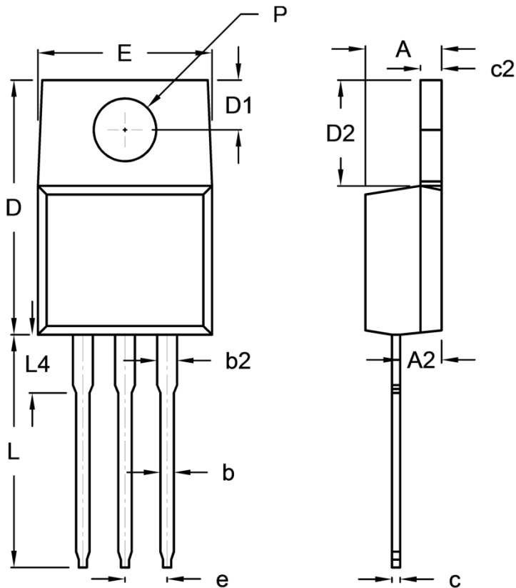
TO-220AB
