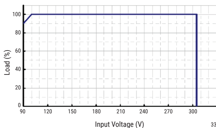
Derating Curve
