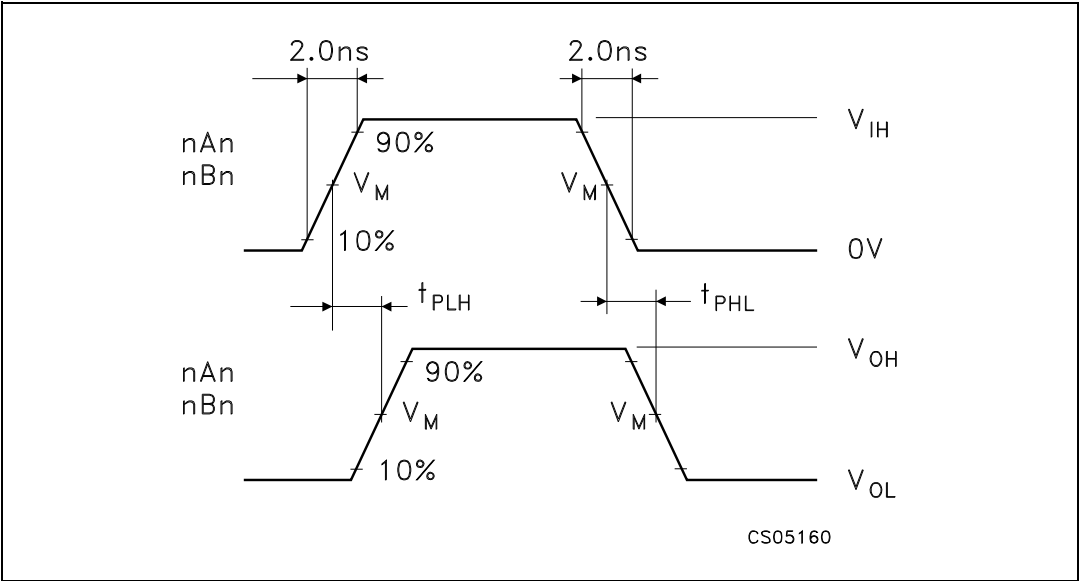
Figure 5. Waveforms - propagation delay (f = 1 MHz; 50% duty cycle)
