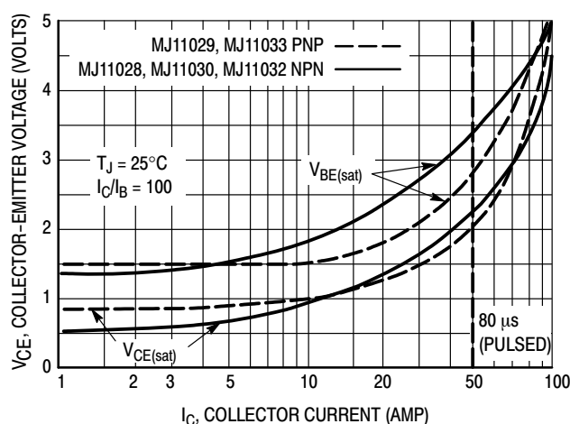
Figure 4. "On" Voltage
