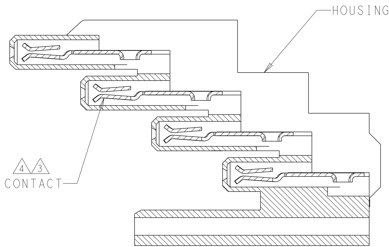
SECTION Z-Z
