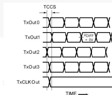
Figure 11. Transmitter Outputs Channel-to-Channel Skew
