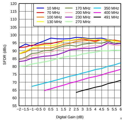
Figure 20. Spurious-Free Dynamic Range vs Digital Gain
