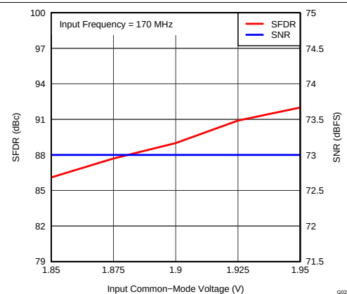
Figure 25. Performance vs Input Common-Mode Voltage (170 MHz)
