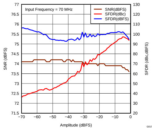
Figure 22. Performance vs Input Amplitude (70 MHz)
