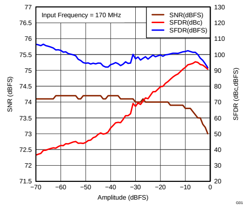
Figure 23. Performance vs Input Amplitude (170 MHz)
