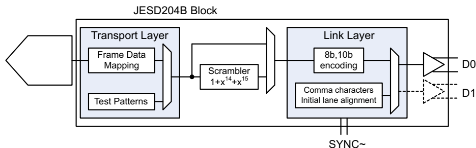
Figure 47. JESD204B Block
