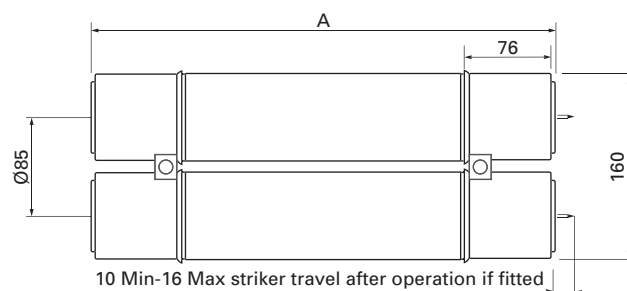
K Tags (double barrel fuse links)
