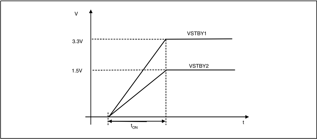
Figure 5. SLEW function
