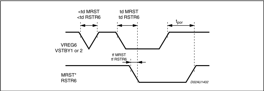
Figure 4. Reset timing
