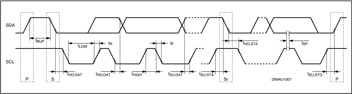
Figure 7. Definition of timing on the I 2 C Bus.
