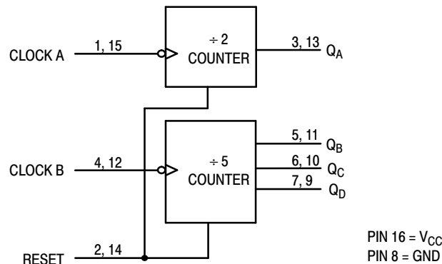
Figure 2. Logic Diagram
