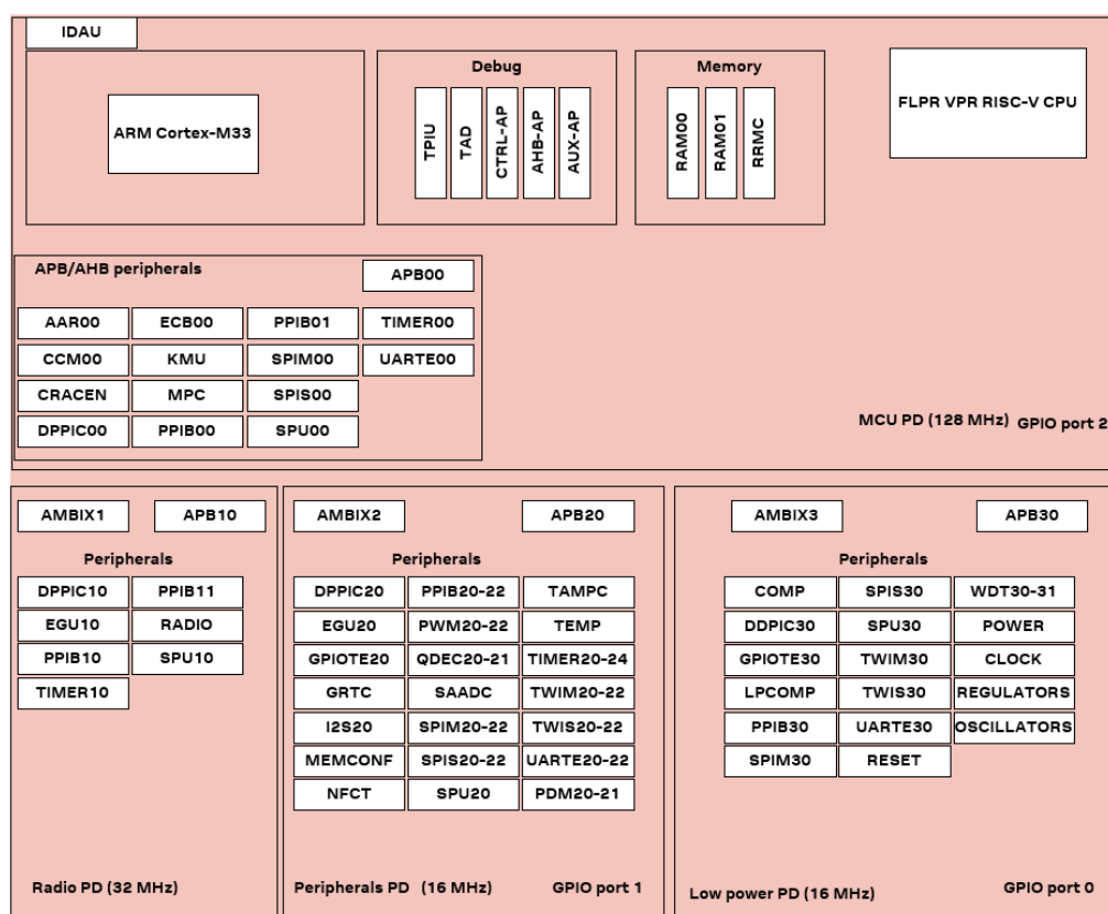
Figure 2: Power domains
