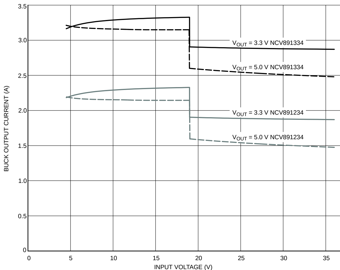
Figure 6. Worst Case NCV891x34 Load Current Capability with a 2.2 µH Inductor
