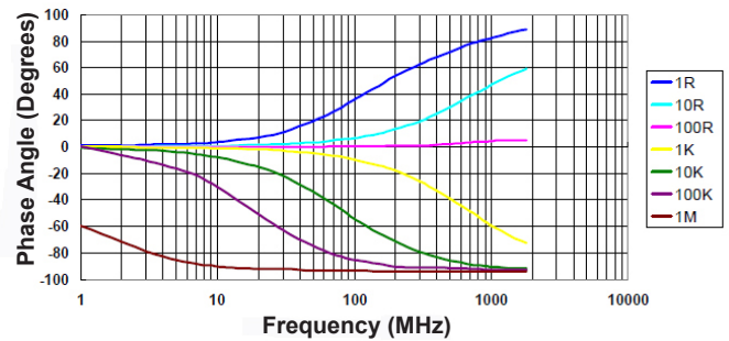
NFR0207 Phase Angle vs. Frequency
