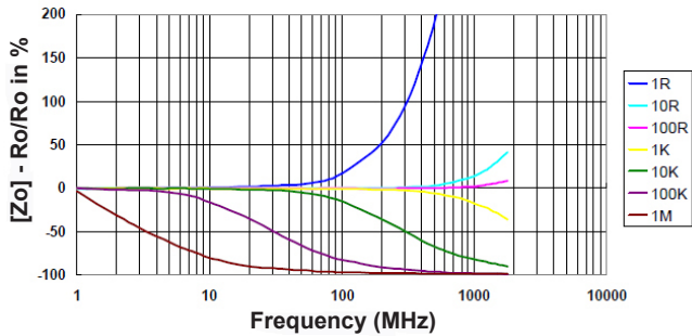
NFR0204 Impedance vs. Frequency
