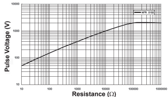
NFR0102 1.2/50 \mu s Lightning Surge
