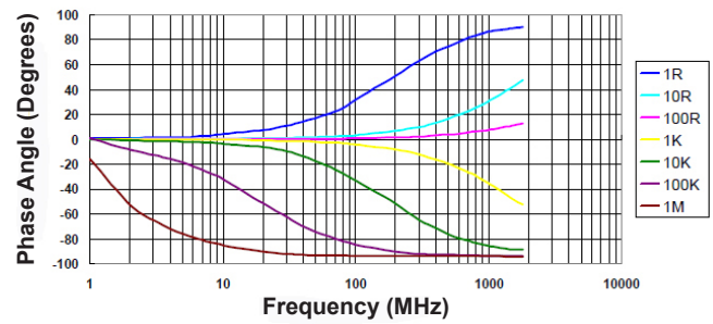
NFR0204 Phase Angle vs. Frequency
