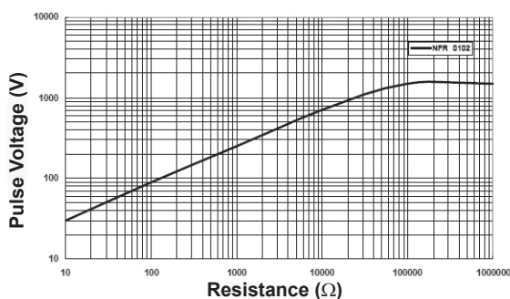
NFR0102 10/700 \mu s Lightning Surge
