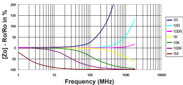
NFR0207 Impedance vs. Frequency
