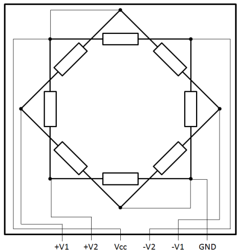
Figure 1: Circuit Diagram
