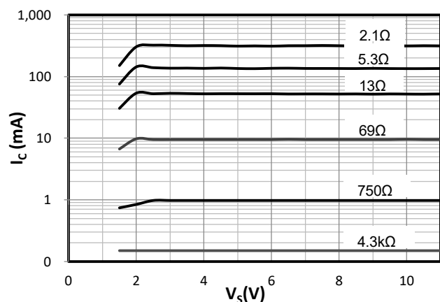
Figure 5. I_C vs. V_S
