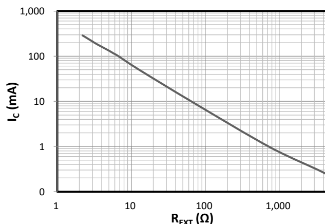
Figure 4. I_C vs R_{EXT}
