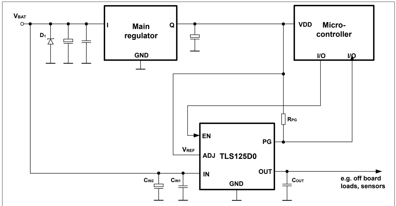
Figure 3 Application diagram
