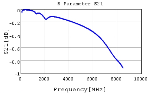
GRM1885C2A151JA01 S21 DCOV, 25degC
