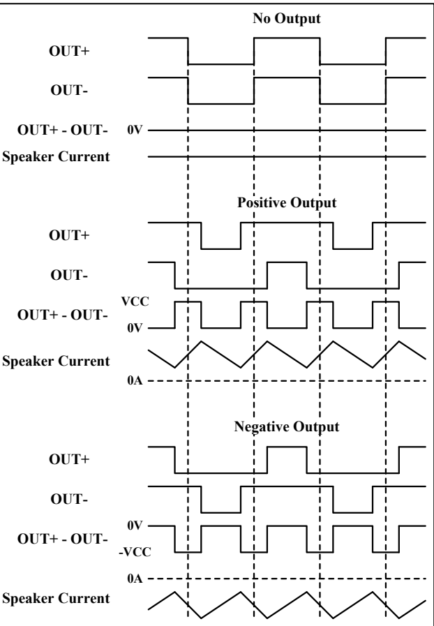
Figure 16 Output Modulation
