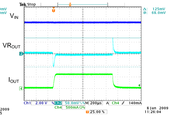
Load Transient Response ( V_{IN}=5.5V , I_{OUT}=10mA \sim 600mA )
