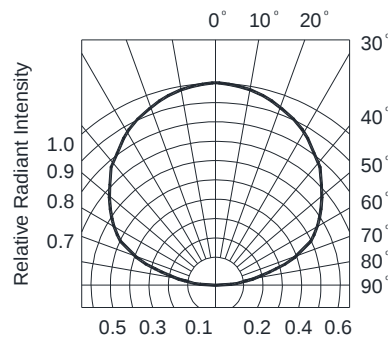
FIG.6 SENSITIVITY DIAGRAM
