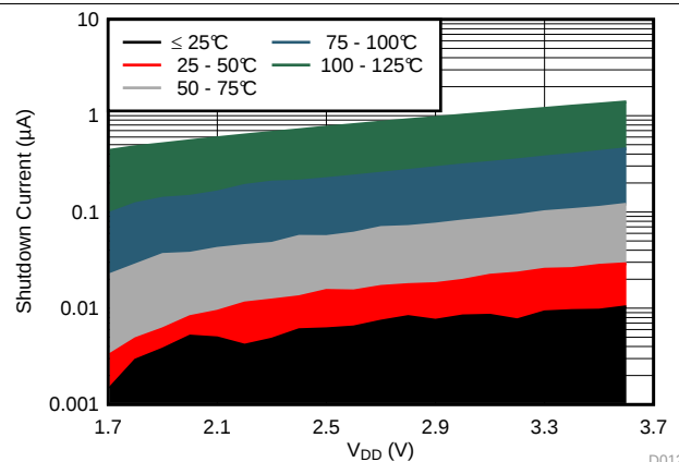
Figure 14. I_{\text{SD}} vs. V_{DD}
