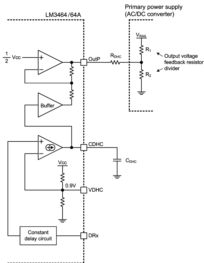
Figure 15. Circuitry of the DHC Mechanism
