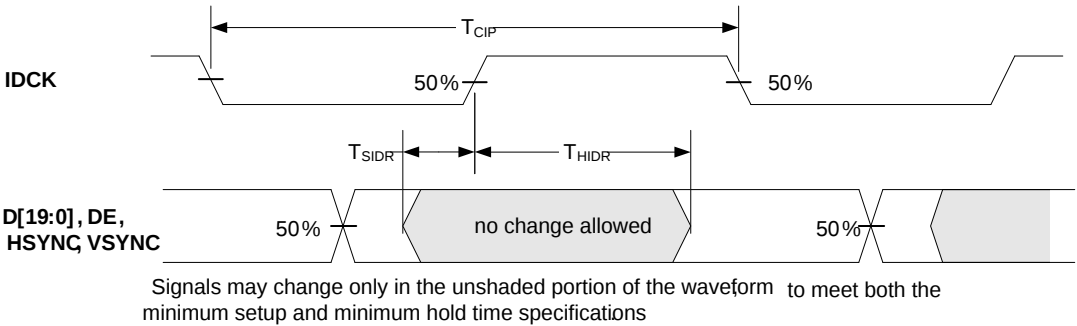
Figure 4.2. Control and Data Single-Edge Setup and Hold Times—EDGE = 1
