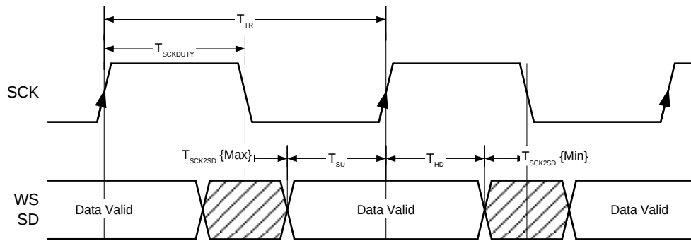
Figure 4.11. I²S Output Timing
