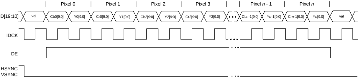
Figure 6.16. 10-bit Color Depth YC Mux 4:2:2 Timing (DRA = 0)
