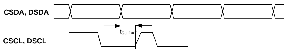
Figure 4.8. I 2 C Data Setup Time
