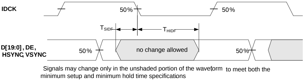
Figure 4.3. Control and Data Single-Edge Setup and Hold Times—EDGE = 0
