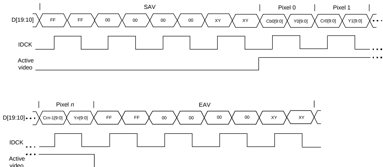
Figure 6.34. 10-bit Color Depth YC Mux 4:2:2 Embedded Sync Dual Edge Timing (DRA = 0, YCSWAP = 0)
