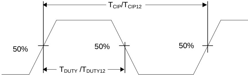
Figure 4.1. IDCK Clock Duty Cycle
