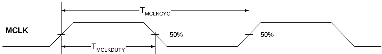
Figure 4.13. MCLK Timing
