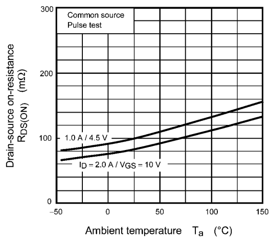
Fig. 8.5 R_{DS(ON)} - T_a
