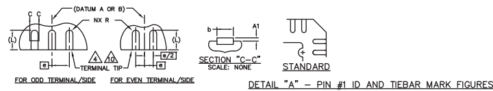
Figure 3. Package Dimensions
