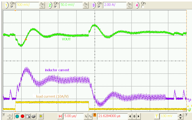
Figure 27. Load Transient, 3.6\text{ V}_{IN} , 1.2\text{ V}_{OUT} , 0.3\text{--}3\text{ A} , 100\text{ ns} Edge, C_{OUT} = 4 \times 22\text{ }\mu\text{F}
