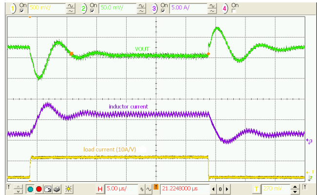
Figure 28. Load Transient, 3.6\text{ V}_{IN} , 1.2\text{ V}_{OUT} , 1.5\text{--}6\text{ A} , 100\text{ ns} Edge, C_{OUT} = 4 \times 22\text{ }\mu\text{F}
