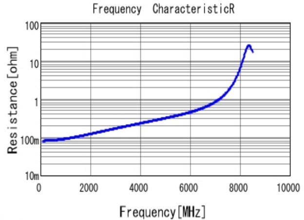
■ GCQ1555C1H7R6WB01 R DC0V, 25degC
