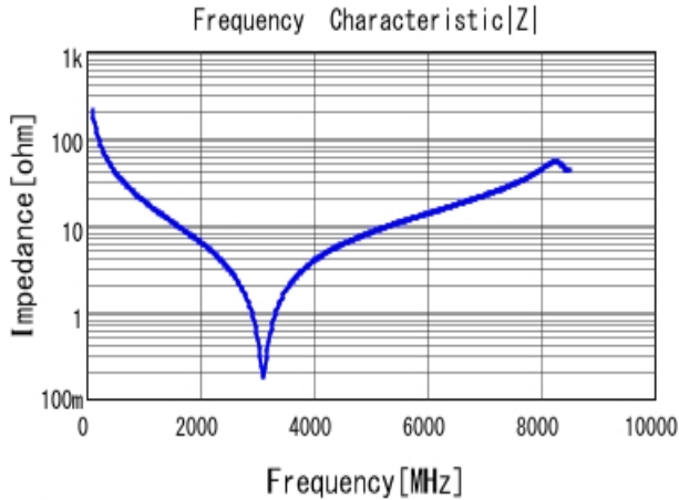
■ GCQ1555C1H7R6WB01 |Z| DC0V, 25degC
