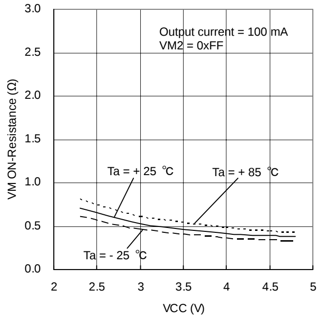
Figure 5. VM ON-Resistance
