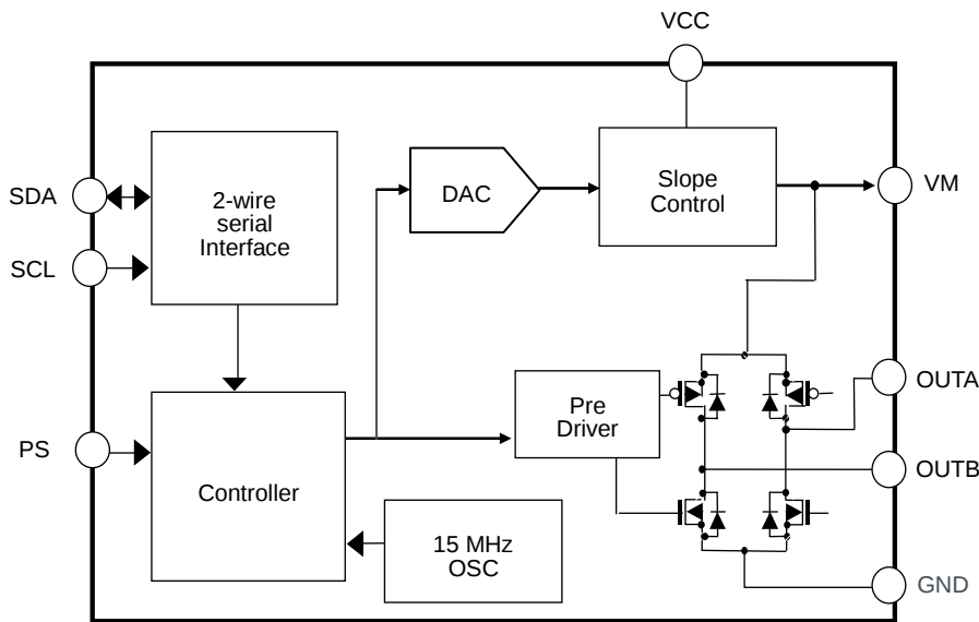
Figure 3. Block Diagram
