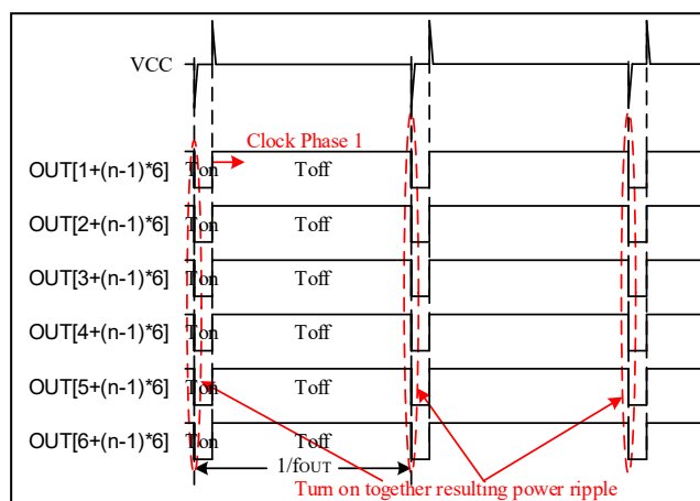
Figure 12 PSn = "0" Clock Phase disable
