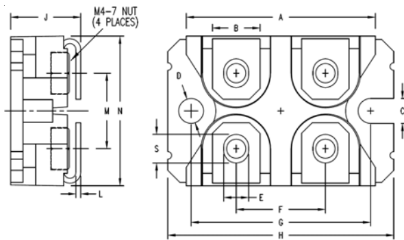
SOT-227B (IXFN) Outline
