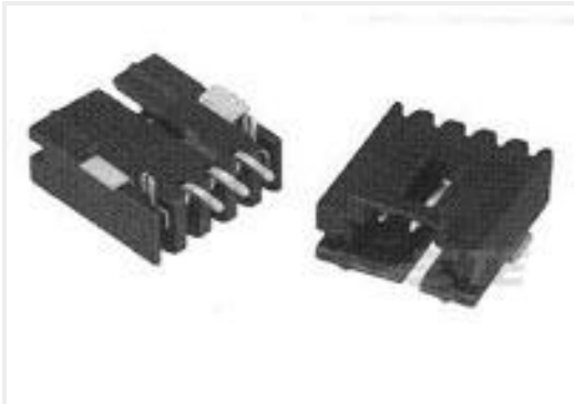
TE Part #5-147278-7 08 MTE HDR SRRA SFMNT .100CL
