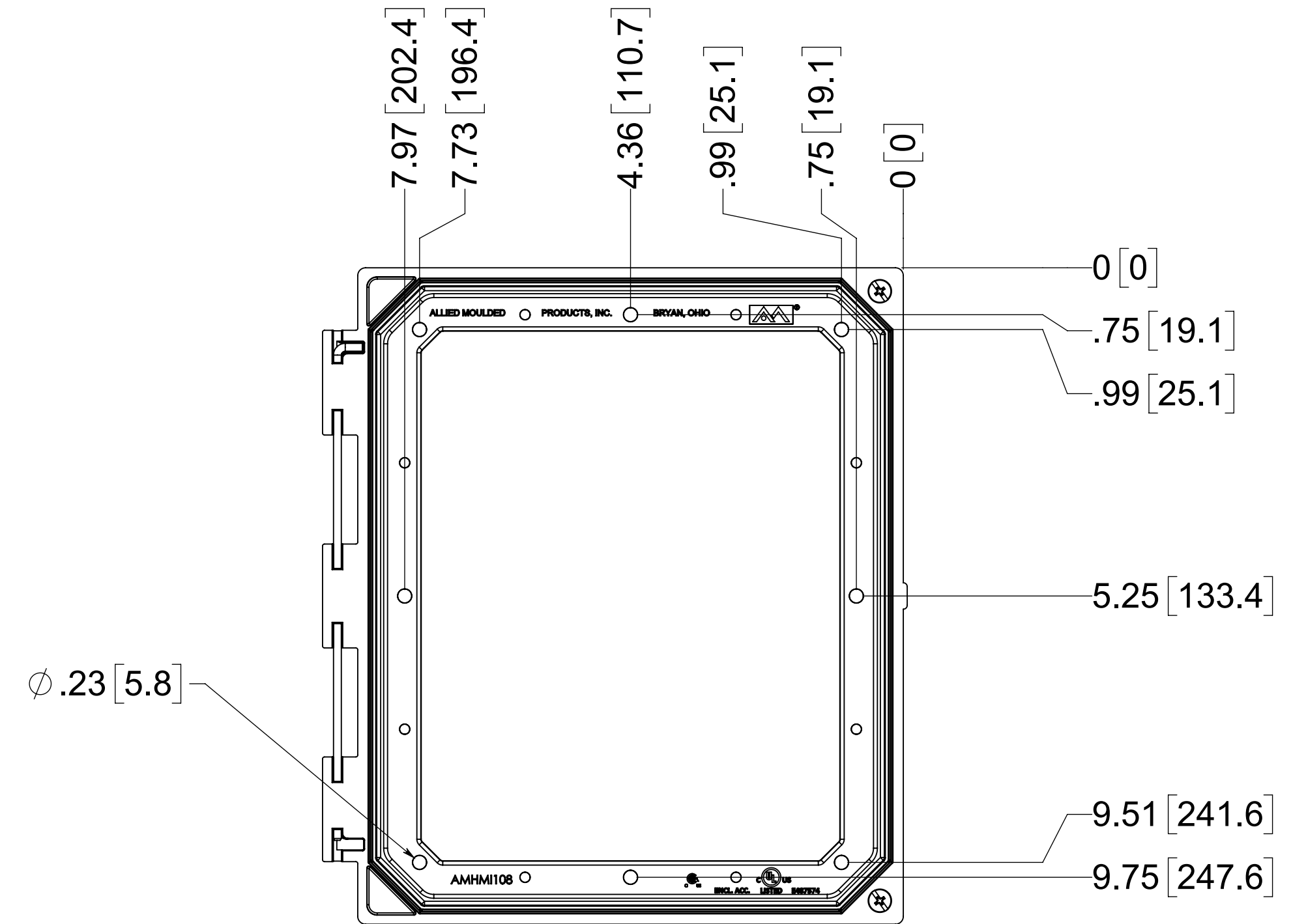
MOUNTING HOLE PATTERN HMI108
