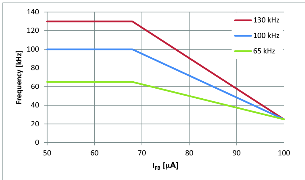
Figure 45. By Observing the Current on the FB pin, the Controller Reduces its Switching Frequency for an Improved Performance at Light Load
