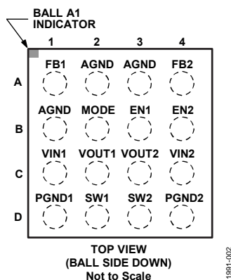
Figure 2. Pin Configuration
