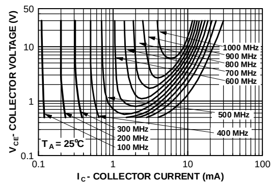
Contours of Constant Gain Bandwidth Product ( f_T )
