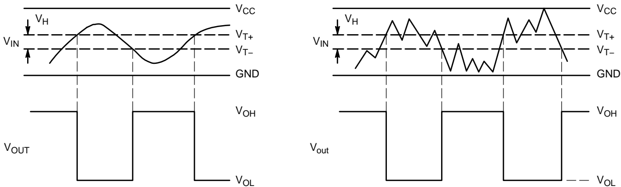
(a) A Schmitt-Trigger Squares Up Inputs With Slow Rise and Fall Times (b) A Schmitt-Trigger Offers Maximum Noise Immunity
