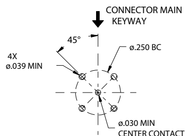
RECOMMENDED CO-AX PCB LAYOUT
