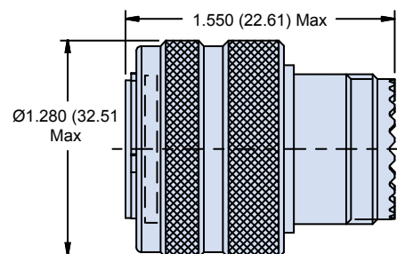
Plug
