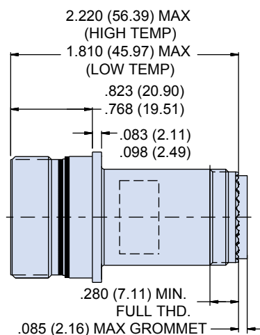
In-Line Receptacle
