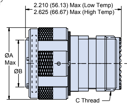
Plug
