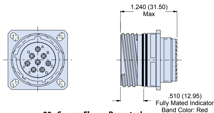
00 - Square Flange Receptacle with Slotted Holes
