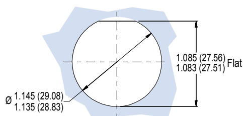
Jam Nut Panel Mounting
