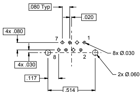
Recommended PCB Layout (Solder Side Of Board)
