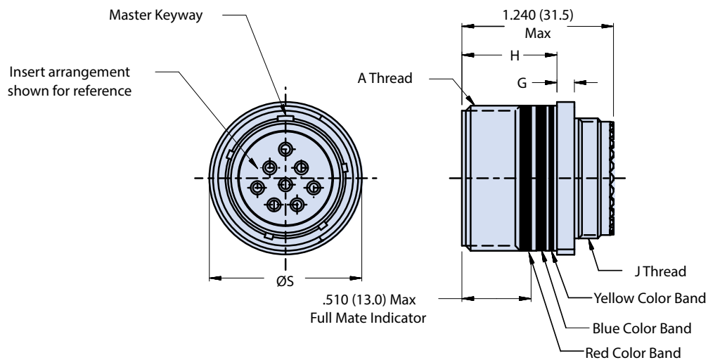
05 - IN-LINE RECEPTACLE
