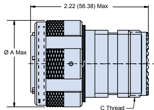
Plug Connector
