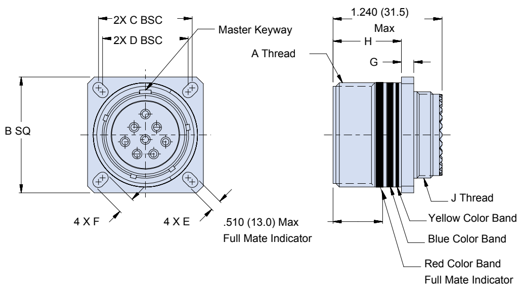
S7 - WALL MOUNT RECEPTACLE WITH SQUARE FLANGE AND SLOTTED HOLES
