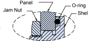
Detail A
