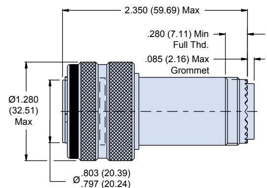
Plug
