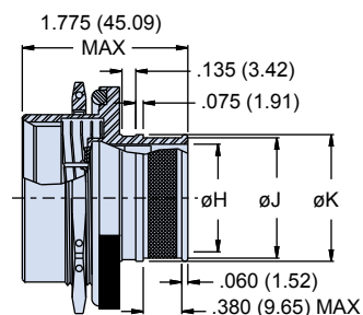
B, SINGLE BAND AND BOOT GROOVE
