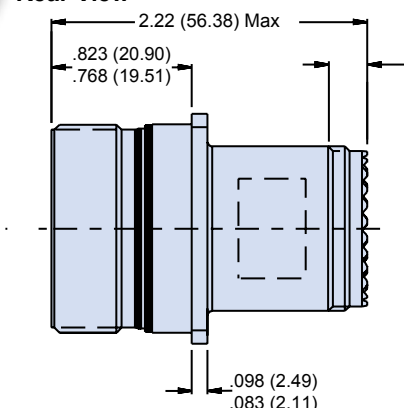
Square Flange Mount Receptacle
