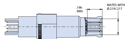
SIZE #8 EL OCHITO SOCKET, PC TAIL DETAIL
