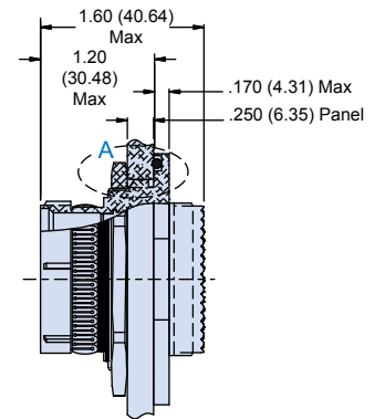
Accessory Thread and Teeth
