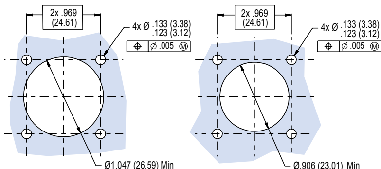
Back Panel Mounting
