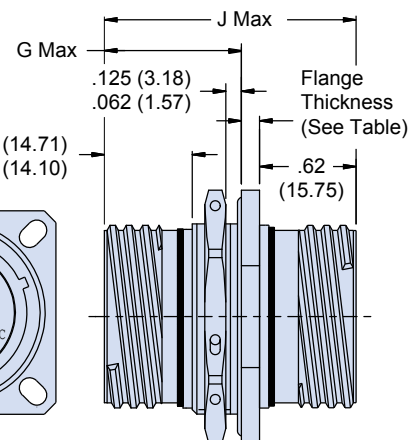
07 - Jam Nut Mount Receptacle
