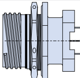
240-383E Dual Flange Jam Nut Receptacles with PC Tails
