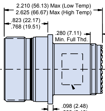
Inline
