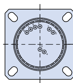
Receptacle Rear View Size #22 Crimp
