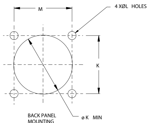
RECOMMENDED MOUNTING HOLES FOR BOX MOUNT RECEPTILES
