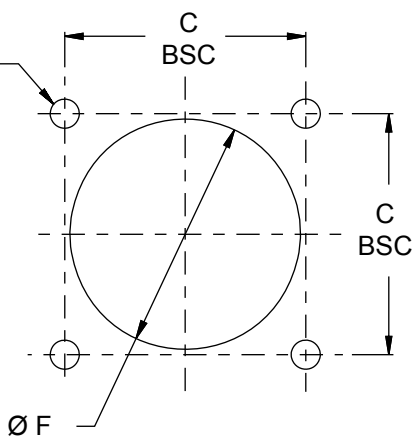
Square Flange Front Panel Mount
