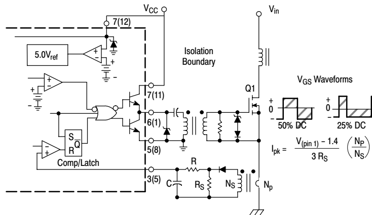
Figure 30. Isolated MOSFET Drive
