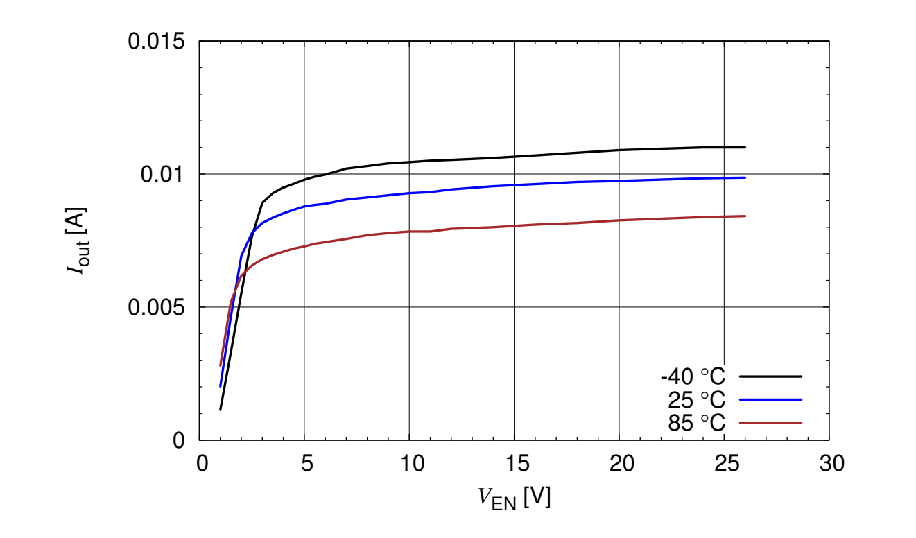
Figure 3-9 BCR 420U: Output Current versus V_{EN} I_{out} = f(V_{EN}) , V_{out} = 2\text{ V} , R_{ext} = \text{open} , T_A = \text{Parameter}
