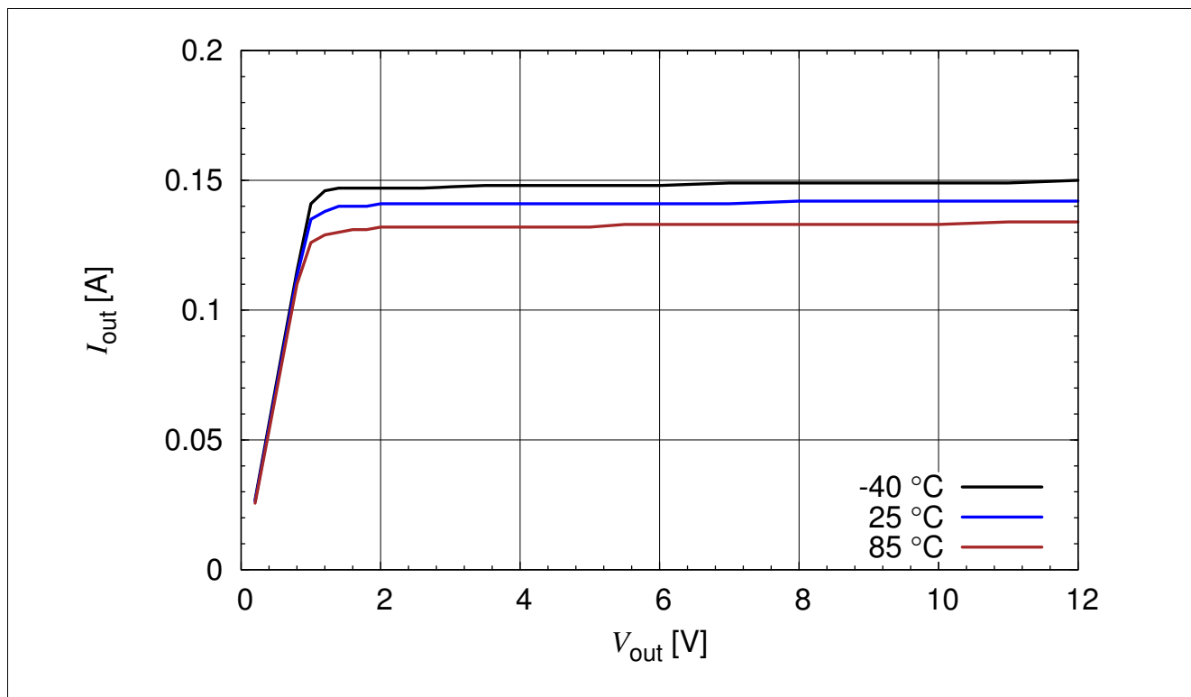
Figure 3-8 BCR 420U: Output Current versus V_{out} I_{out} = f(V_{out}) , V_{EN} = 40\text{ V} , R_{ext} = 6\ \Omega , T_A = \text{Parameter}
