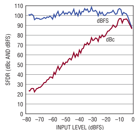
LTC2141-12: SFDR vs Input Level, f_{IN} = 70\text{MHz} , 40\text{Mpsps} , 2\text{V} Range
