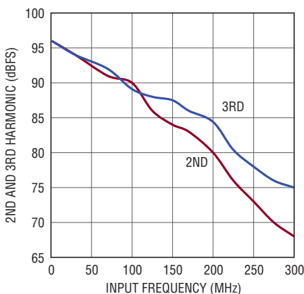
LTC2141-12: 2nd, 3rd Harmonic vs Input Frequency, -1\text{dBFS} , 40\text{Mpsps} , 2\text{V} Range
