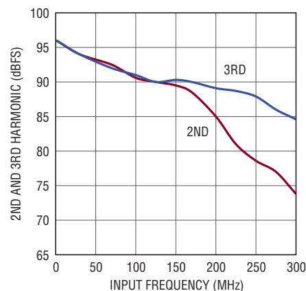
LTC2141-12: 2nd, 3rd Harmonic vs Input Frequency, -1\text{dBFS} , 40\text{Mpsps} , 1\text{V} Range
