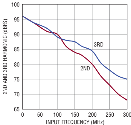
LTC2140-12: 2nd, 3rd Harmonic vs Input Frequency, -1\text{dBFS} , 25\text{Mps} , 2\text{V} Range
