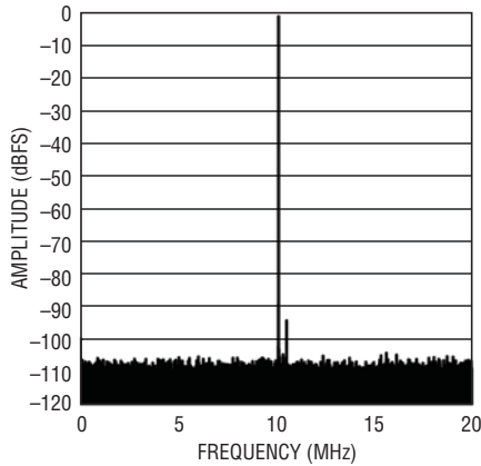
LTC2141-12: 64k Point FFT, f_{IN} = 30\text{MHz} , -1\text{dBFS} , 40\text{Mpsps}
