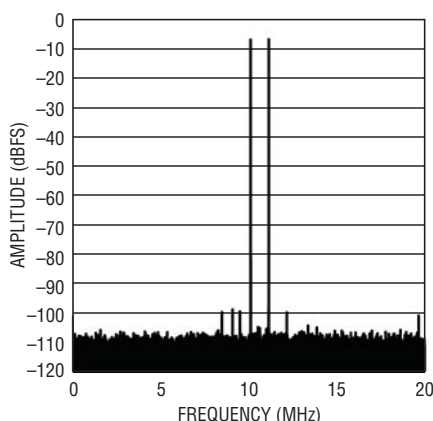
LTC2141-12: 64k Point 2-Tone FFT, f_{IN} = 69\text{MHz} , 70\text{MHz} , -7\text{dBFS} , 40\text{Mpsps}
