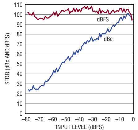
LTC2140-12: SFDR vs Input Level, f_{IN} = 70\text{MHz} , 25\text{Mps} , 2\text{V} Range
