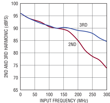
LTC2140-12: 2nd, 3rd Harmonic vs Input Frequency, -1\text{dBFS} , 25\text{Mps} , 1\text{V} Range
