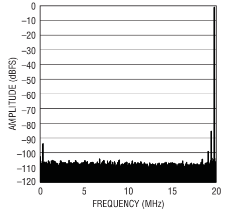
LTC2141-12: 64k Point FFT, f_{IN} = 140\text{MHz} , -1\text{dBFS} , 40\text{Mpsps}
