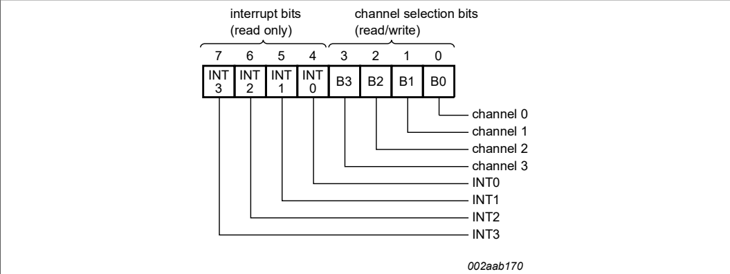
Figure 6. Control register
