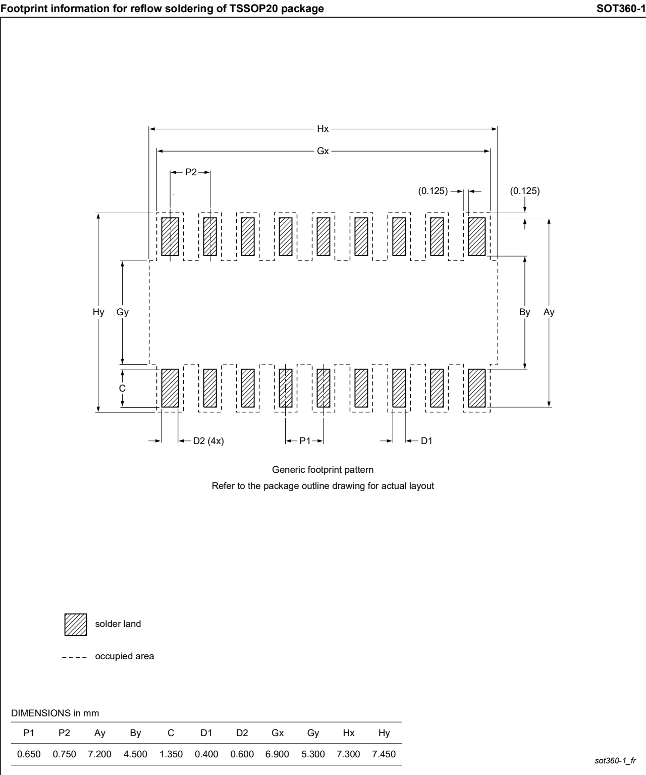
Figure 26. PCB footprint for SOT360-1 (TSSOP20); reflow soldering
