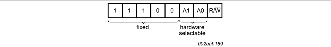
Figure 5. Target address PCA9545A
