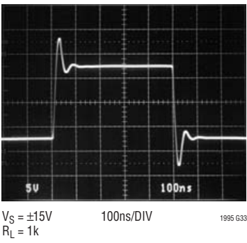
Large-Signal Transient ( G = 1 )
