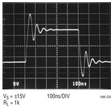
Large-Signal Transient (Noninverting, G = 1 , C_L = 100pF )
