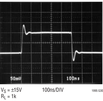
Small-Signal Transient ( G = 1 )
