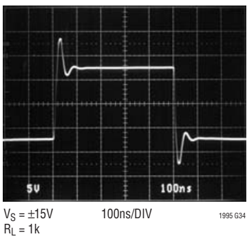
Large-Signal Transient ( G = -1 )
