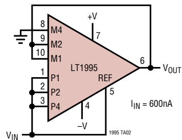
High Input Impedance Precision Gain of 2 Configuration
