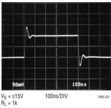
Small-Signal Transient ( G = -1 )
