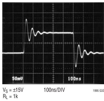
Small-Signal Transient (Noninverting, G = 1 , C_L = 100pF )
