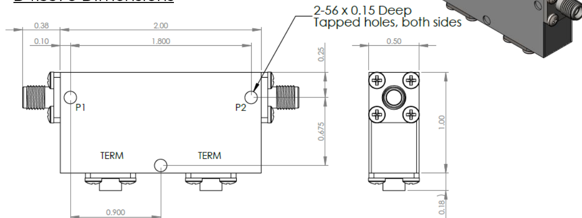
D4I3570-3 Dimensions
