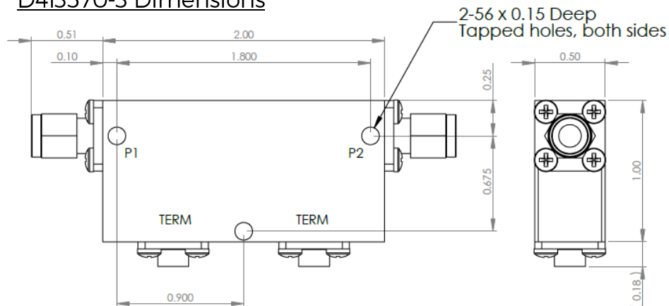
D4I3570-3 Dimensions
