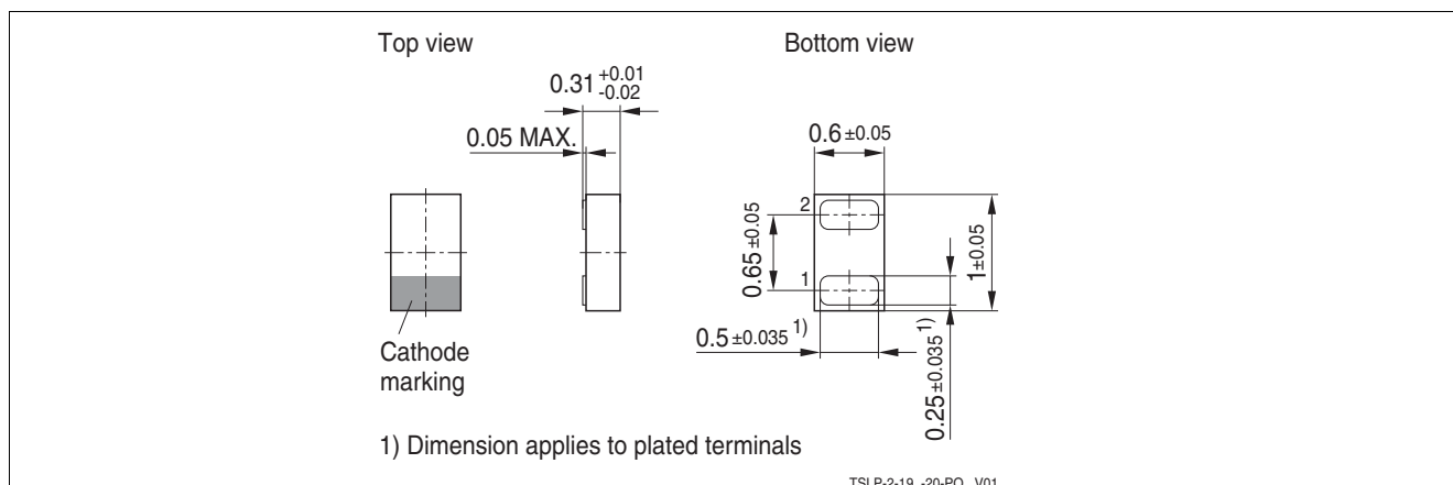
Figure 5-1 TSLP-2-19: Package overview (dimension in mm)
